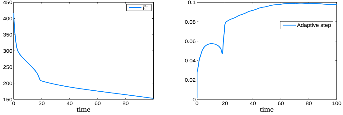
Figure 3: Evolutions of energy (left) and time steps (right) of the Allen-Cahn equation using adaptive time strategy until final time T = 100 .
