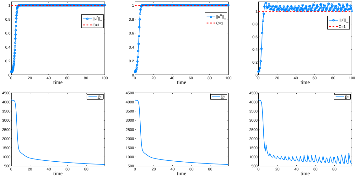
Figure 4: Maximum norm (top) and energy (bottom) of the Allen-Cahn equation using different time steps \tau = 0.2, 0.4, 0.8 (from left to right), respectively.
