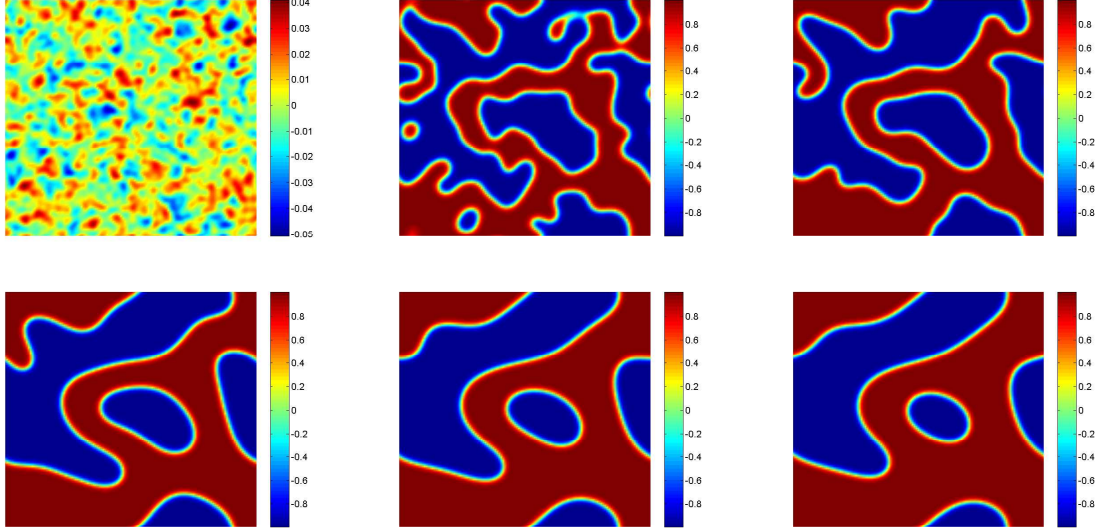
Figure 5: Solution snapshots of coarsening dynamics of Allen-Cahn equation using adaptive time strategy at t = 1, 10, 20, 50, 80, 100 , respectively.
