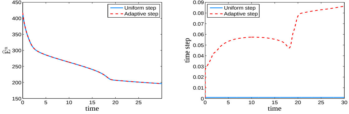
Figure 1: Evolutions of energy (left) and time steps (right) of the Allen-Cahn equation using different time strategies until time T = 30 .
