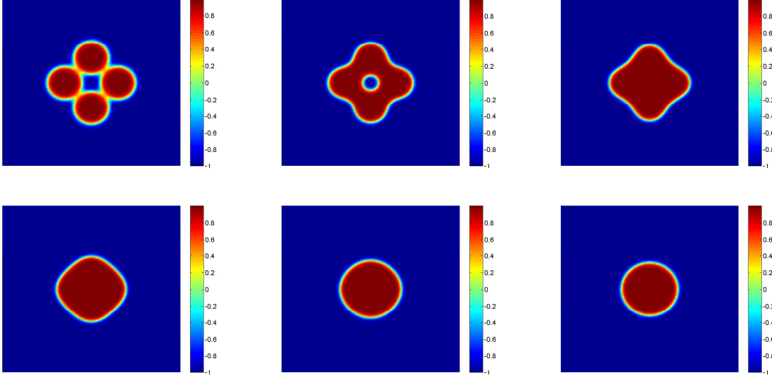
Figure 2: Solution snapshots of the Allen-Cahn equation using adaptive time strategy at t = 1, 10, 20, 50, 80, 100 , respectively.
