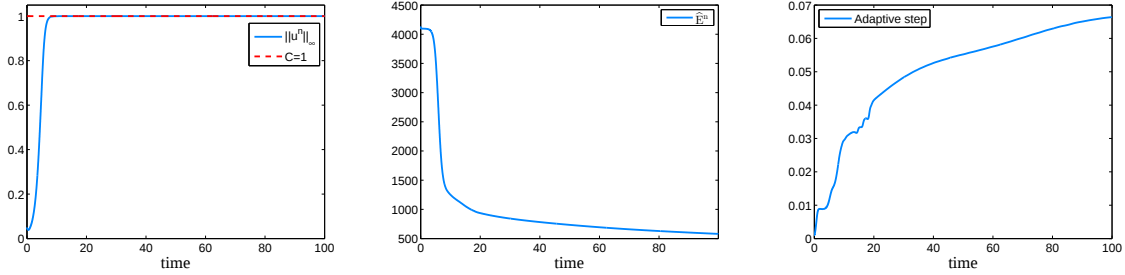
Figure 6: Evolutions of Maximum norm (left), energy (middle) and adaptive time steps (right) of coarsening dynamics of Allen-Cahn equation using adaptive time strategy.
