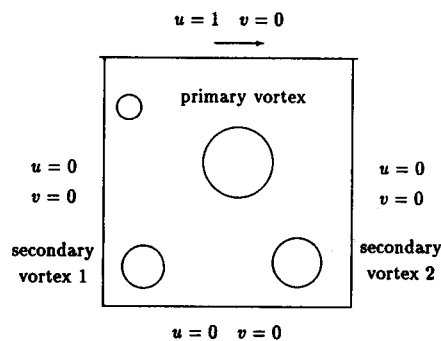
Figure 2. Driven cavity
