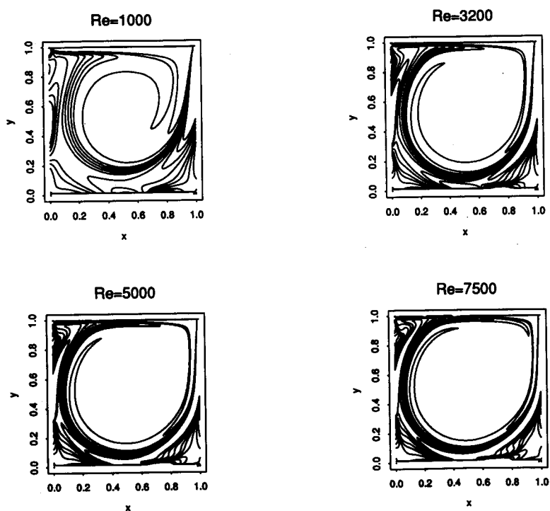
Figure 8. Vorticity contours for Re=1000, 3200, 5000 and 7500 using a 129 \times 129 uniform grid
