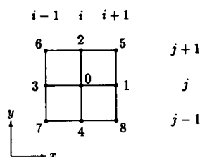
Figure 1. Computational stencil
